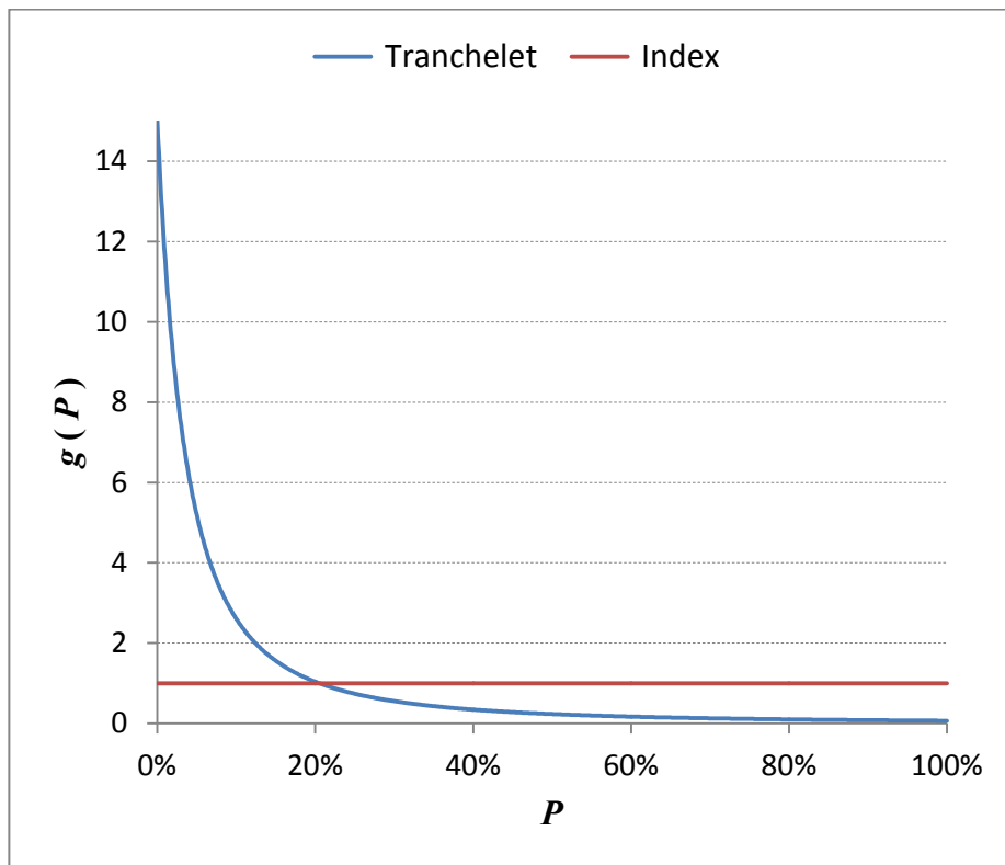
Figure 3: Delta assumed by the SA-CCR for infinitesimally thin tranches.
