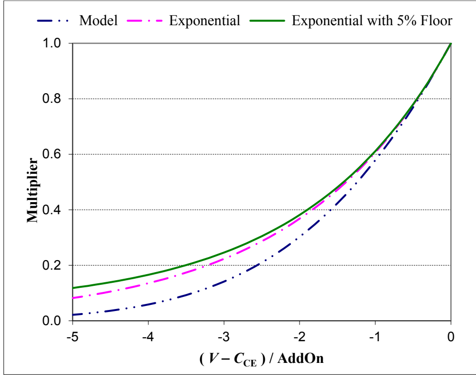
Figure 1: The dependence of multiplier on (V - C_{\text{CE}}) / \text{AddOn}
