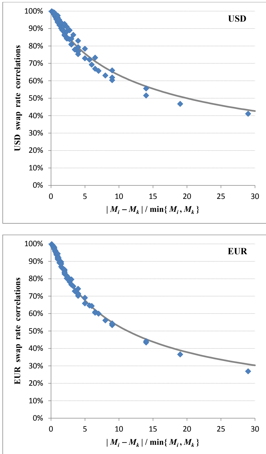
Figure 2: Swap rate correlations and the parametric fitting function for G4 currencies
