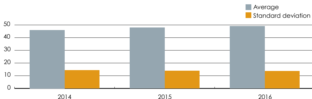
Figure 2: Convergence of scores, mean and variance—2014, 2015 and 2016
